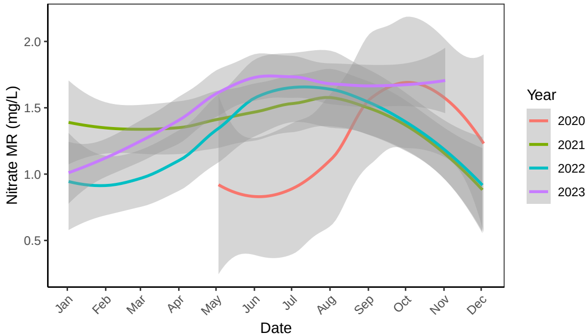
B2 Raceway 1 Nitrate MR (mg/L) Monthly Mean
